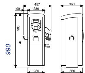
Tank Version
