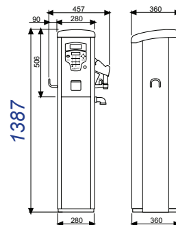
Column Version
