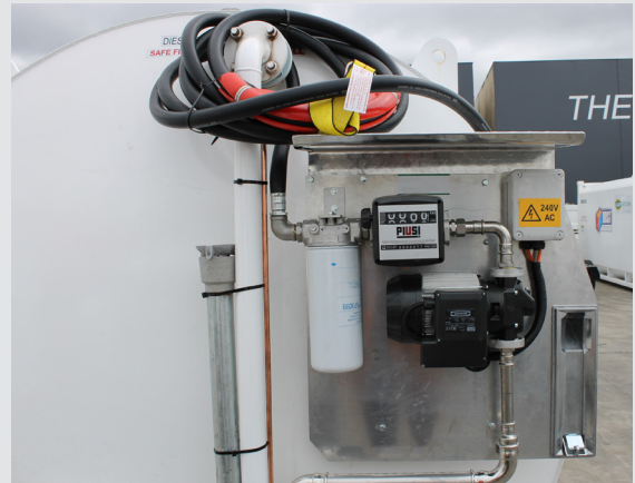
RTR Rural Farm Tanks with various Fuel Dispensing Systems
